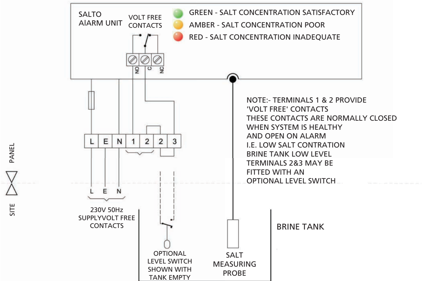
The salt measuring probe
